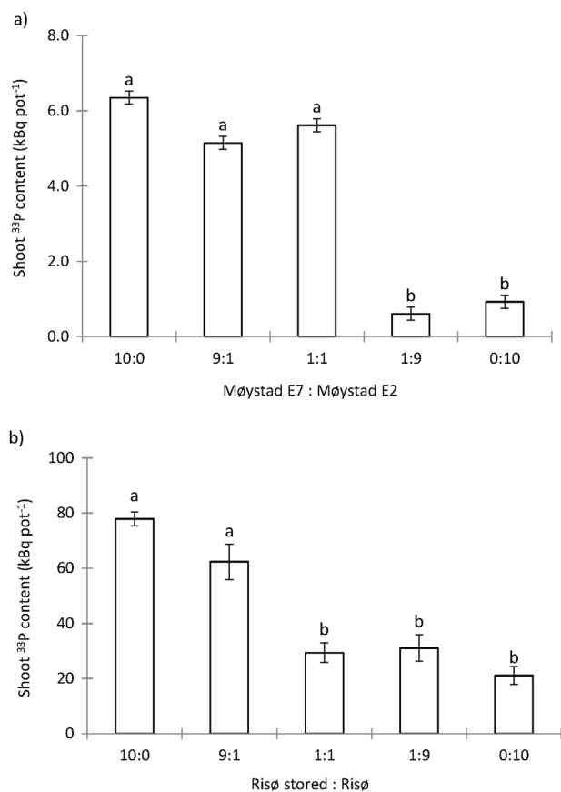
Fig. 5 Shoot ^{33}\text{P} uptake from HCs containing (a) either Møystad E2 or Møystad E7 soil, or three different mixes of the two soils and (b) either Risø stored or Risø soil, or three different mixtures of the two soils. Root external mycelium grew from M. truncatula roots colonised by R. irregularis (Expt. 3)
