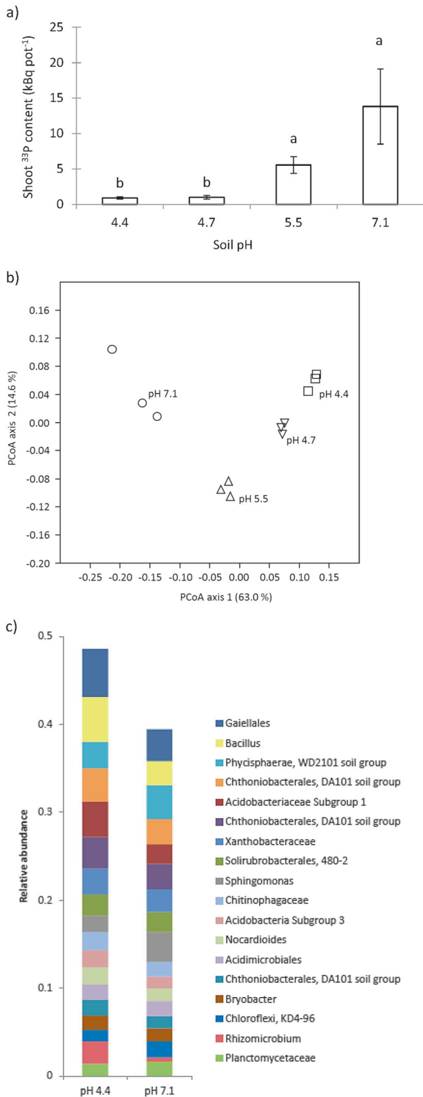
Fig. 3 Shoot 33 P uptake (a) and principal coordinates analysis (PCoA) of bacterial communities (b) from the HC containing unsterile Møystad E2 soil, amended with increasing amounts of CaCO 3 to increase soil pH (Expt. 3). The PCoA was made on Bray–Curtis dissimilarities of OTUs with 97% similarity. The relative abundance of genus- or higher-level taxa (c) in Møystad E2 soils with pH 4.4 or 7.1 (Expt. 3). Only taxa constituting >1.5% of total abundance in the two soils are included in the bar plot
