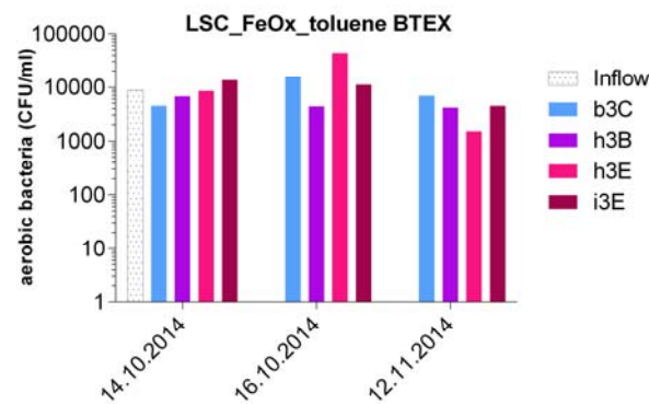
Figure 4: Colony Forming Units (CFU/mL) of aerobic bacteria in LSC water samples. Note the logarithmic scale. Anaerobic bacteria were cultivated as well, but no colony was found.
