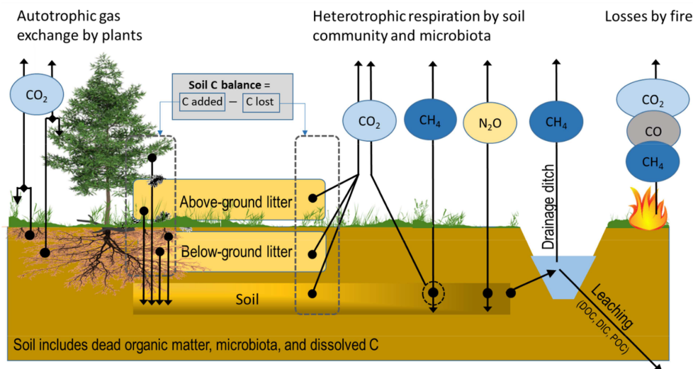
Figure 1. CO 2 , CH 4 and N 2 O fluxes and mass transfer components contributing to soil C-stock changes in a forest ecosystem on drained organic soil, as in IPCC (2014). Arrows indicate flux/transfer direction.
