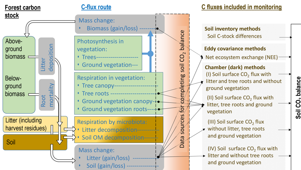
Figure 2. Forest C stock, processes resulting in changes in the dead organic matter C stock in soil, C fluxes typically monitored (see also Sect. S1, Table S1) and complementary data sources needed for forming soil CO 2 balance estimates (black arrows) in incomplete flux monitoring set-ups, according to IPCC (2014). Numbers I–IV next to monitoring set-ups by dark chambers refer to respective studies listed in Sect. S1, Table S1. Waterborne C losses and losses by fires are excluded from the figure.
