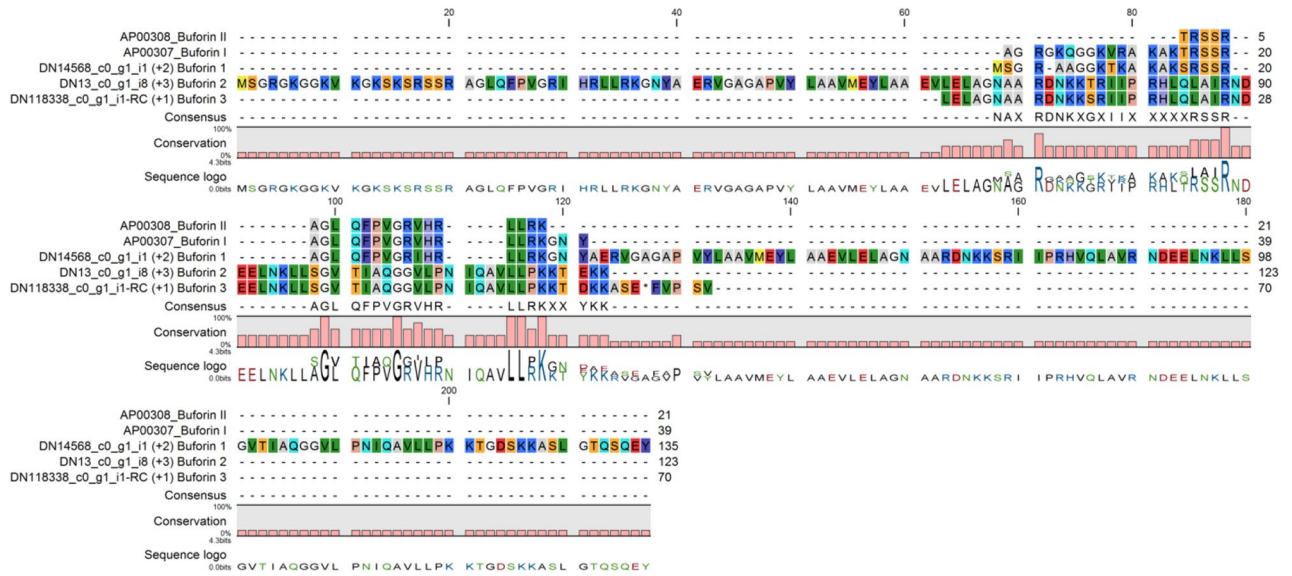
Figure 1. Alignments of the red king crab buforins with published data, Buforin 1 (AP00307) and Buforin II (AP00308).
