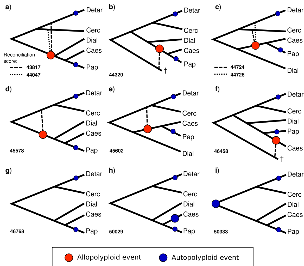
FIGURE 4. Hypotheses involving allopolyplody derived from GRAMPA and their reconciliation scores compared to hypotheses involving only autopolyplody. (a)–(f) All eight allopolyplody hypotheses that gave lower (better) reconciliation scores than (g), which represents the null hypothesis with no allopolyplody. Hypotheses involving an additional autopolyplody event in Caesalpinoideae (h), or at the legume crown node (i), lead to higher (worse) reconciliation scores. Large circles indicate putative allo- or autopolyplody events accounted for in the analysis (as per the legend), small circles indicate autopolyplody events in Papilionoideae and Detarioideae that were not taken into account and removed from the input gene trees prior to the analysis. Solid lines represent the species tree topology; dashed lines connect to the putative second parental lineage of the allopolyplody, with hypothetical extinct lineages indicated with a †. Caes = Caesalpinoideae, Cerc = Cercidoideae, Detar = Detarioideae, Dial = Dialioideae and Pap = Papilionoideae.
