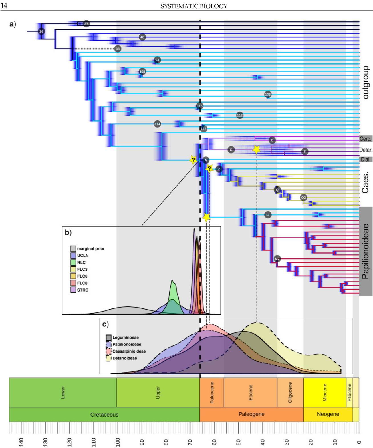
FIGURE 5. The origin of the legumes is closely associated with the KPB. a) Chronogram estimated with eight fixed local clocks (FLC8 model) in BEAST, with the clock partitions indicated by colored branches, from an alignment of 36 genes selected as both clock-like and highly informative and hence well-suited for dating analyses. Blue shading represents 500 post-burn-in trees ("densitree" plot) indicating posterior distributions of node ages. Yellow stars indicate putative legume WGD events, the placement of a putative allopolyploid event is equivocal and is indicated by two stars labeled with question marks (one on the stem lineage of the family and one on the stem lineage of Caesalpinioideae because the time-scaling analysis of gene duplications presented in (c) is based on this subfamily). Labeled circles indicate placements and ages of fossil calibrations listed in Table 1. Note that fossil A is placed on the legume stem node but postdates the median crown age estimates for the family and is therefore not plotted on the legume stem lineage (similar for fossils 27 and 38). b) Prior and posterior distributions for the crown age of legumes under different clock models, as indicated in the legend. c) Density plots of age estimates for duplication nodes in gene trees, for all duplications that mapped onto the legume crown node in the Notung analysis in gray and for duplications in the three well-sampled subfamilies Papilionoideae, Caesalpinioideae, and Detarioideae as indicated in the legend.
