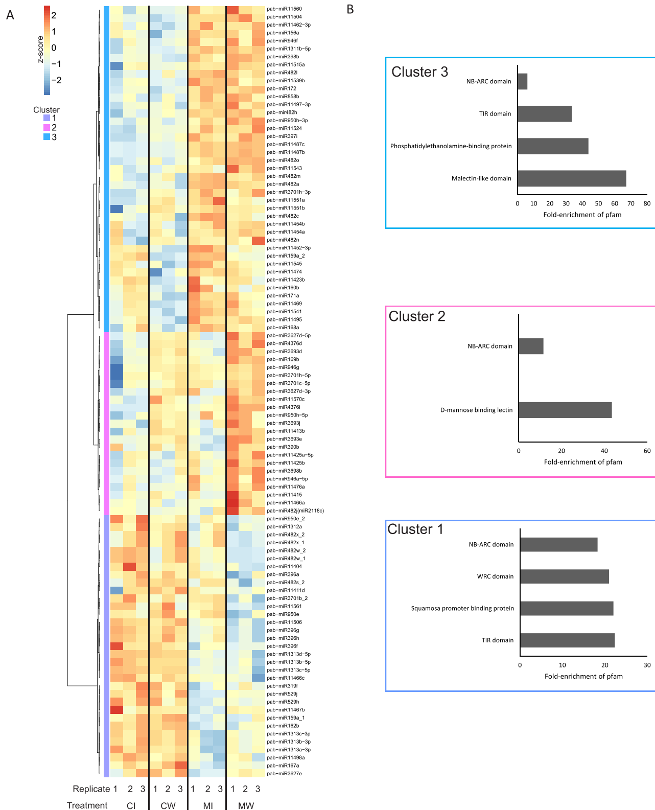
Fig. 5. Clustering of differentially expressed miRNAs and Pfam (protein family) enrichment analysis of their predicted mRNA targets in Norway spruce bark. (A) Heatmap of z-scores of VST counts computed for all miRNAs differentially expressed ( p adjusted < 0.05 ) in at least one of the six pairwise comparisons between the four treatment combinations (see Fig. 1 for an explanation of the experimental design and treatment combinations). Differentially expressed miRNAs clustered into three main expression groups (Cluster 1–3). Cluster 1 = prolonged upregulated. Cluster 2 = primed upregulated. Cluster 3 = prolonged downregulated. (B) Pfam enrichment analysis of each expression cluster showing the top four enriched (or the two enriched in Cluster 2) Pfam categories with an adjusted p -value < 0.05 .
