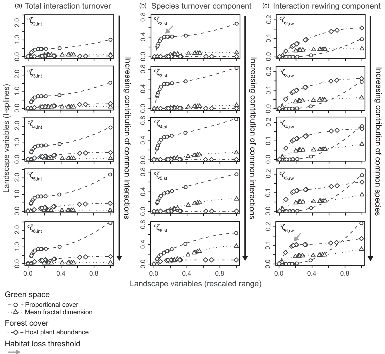
FIGURE 4 Multi-site generalised dissimilarity modelling of interaction turnover: The most important landscape variables explaining (a) total interaction turnover ( c_{int}^z ) and its components, (b) species turnover ( c_{sp}^z ) and (c) interaction rewiring ( c_{rw}^z ). These are shown across increasing orders of zeta diversity (i.e. from the top panel results of pairwise c_2^z to the bottom panel results of multisite, six in this case c_6^z ), interpreted along the arrows to the right. Interpretation of each panel: Each landscape variable is transformed using I-splines scaled from low (right) to high (left) levels of modification for each variable (e.g. low (left) to high (right) green space cover). Points show the location of the sampled sites along the landscape variable gradients. A steep slope indicates a high rate of turnover. Potential critical thresholds for habitat loss are indicated (see further explanation in the main text). Note that the y-axes scales differ between A, B and C. Results are shown for those environmental variables that had high explanatory power, that is, green space proportional cover and fragmentation (mean fractal dimension, D ) and host plant abundance. Variables with low explanatory power and covariates are shown separately in Supporting Information S3, Figure S3.2
