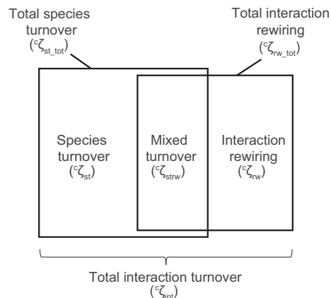
FIGURE 1 Schematic showing how total interaction turnover for multiple sites is partitioned into three components. Total interaction turnover ( ^c\zeta_{int} ) can be partitioned into interaction turnover due to species turnover only ( ^c\zeta_{st} ), interaction turnover due to rewiring only ( ^c\zeta_{rw} ) and turnover due to a mixture of both ( ^c\zeta_{strw} ). Thus, ^c\zeta_{st\_tot} is turnover involving some component of species turnover and ^c\zeta_{rw\_tot} is turnover involving some component of interaction rewiring. For pairwise turnover, there is no overlap between species turnover and interaction rewiring (i.e. no mixed turnover component)
