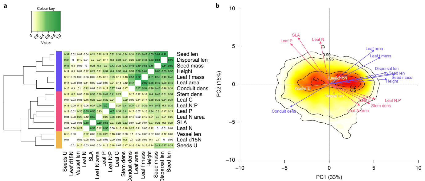
Fig. 1 | Previously identified global axes of variation in size and economics traits hold for an extended trait set ( n = 36,197 species per ecoregion median).
