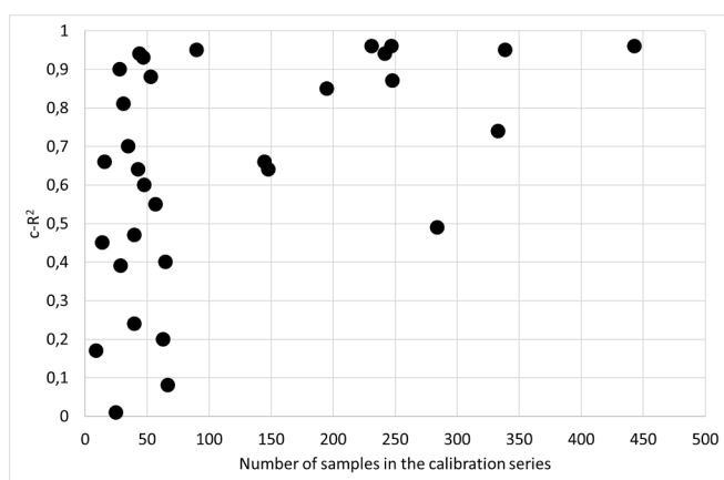
Fig. 3. The relationship between the number of samples in the calibration series and the c-R^2 (the goodness of fit between turbidity and SSC).
