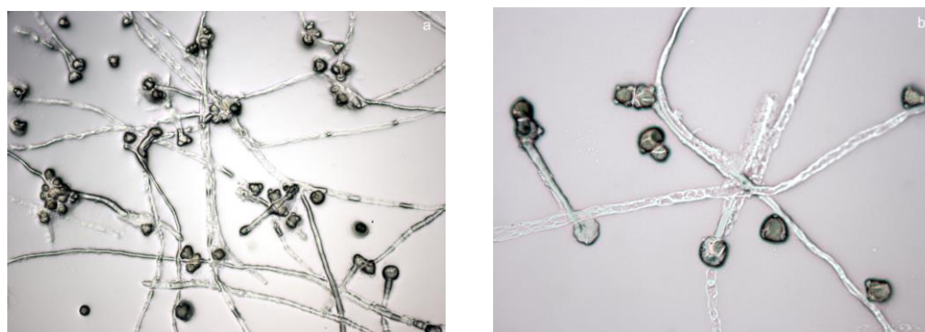
Figure 2. In vitro pollen germination in 'Oblačinska' sour cherry clones II/2 after 24 h of incubation (a) and XI/3 24 h of incubation (b).
