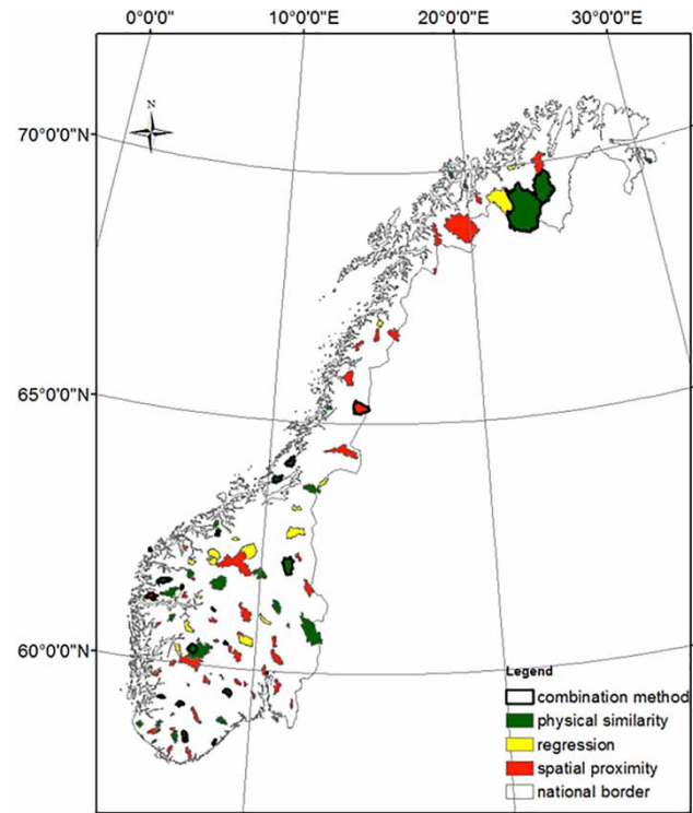
Figure 6 | Spatial distribution of best performing methods. For each catchment, the color indicates which of the three standard regionalization methods (physical similarity, regression, spatial proximity) produced the best results. Catchments where the combination method outperformed the three other methods are highlighted by a thick black border.
