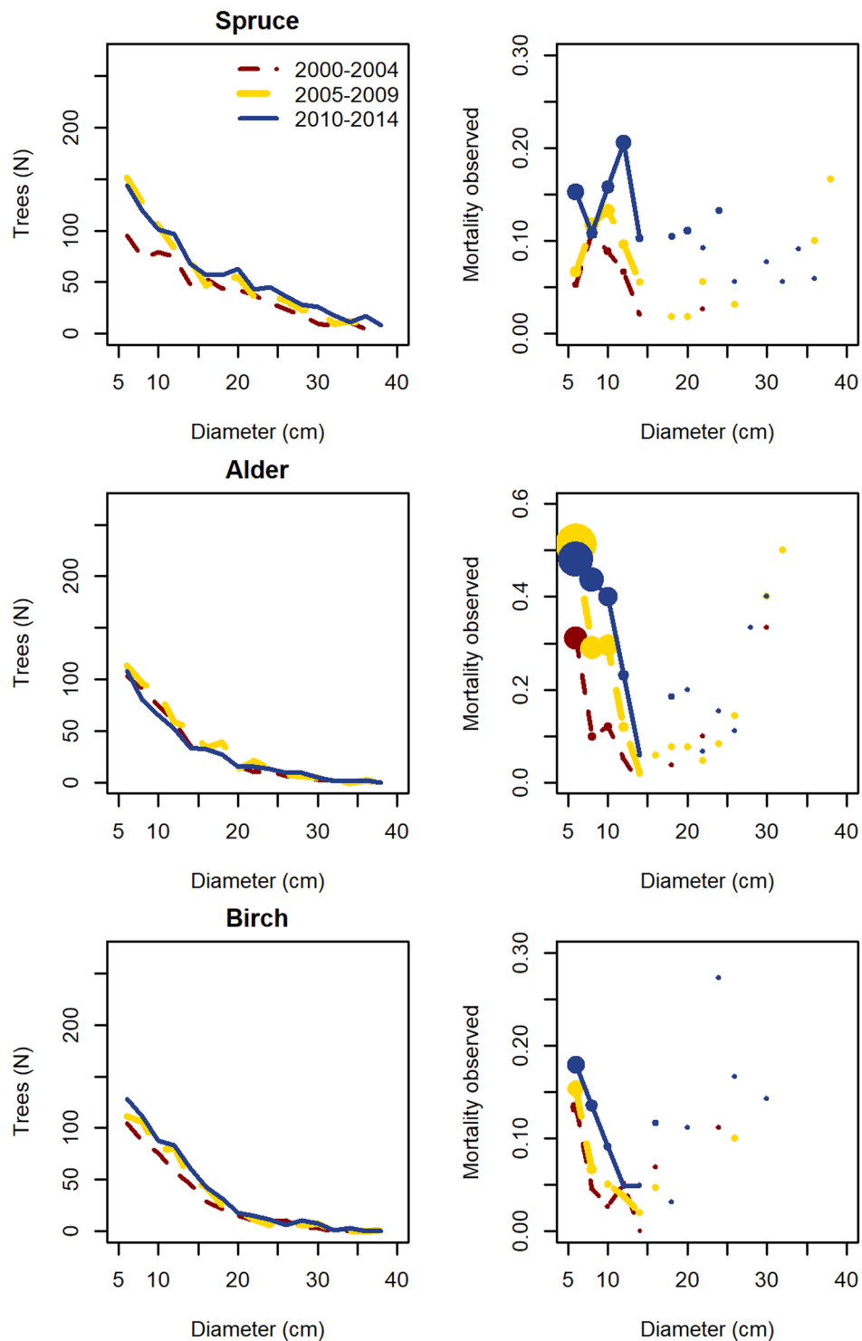
Figure 3. Diameter distribution and observed mortality of other species located in the ash plots. The distributions are presented for the three periods studied (2000–04, 2005–09, 2010–14, corresponding to the 8 th , 9 th and 10 th national forest inventories, respectively) for Spruce, Alder and Birch.
