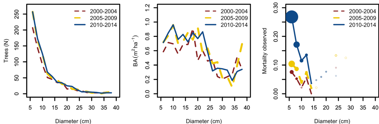
Figure 1. Number of ash trees observed in the Norwegian National Forest Inventory. Left: Trees by diameter class at intervals of 5 cm for the three periods studied (2000–04, 2005–09, 2010–14, corresponding to the 8 th , 9 th and 10 th national forest inventories, respectively). Middle: basal area observed for the same periods. Right: Tree mortality observed for the same periods. In this case, the diameter classes were defined each 2 cm and the size of the points represents the number of trees dead (max N = 71 ). Lines do not link values when there are less than three trees dead.
