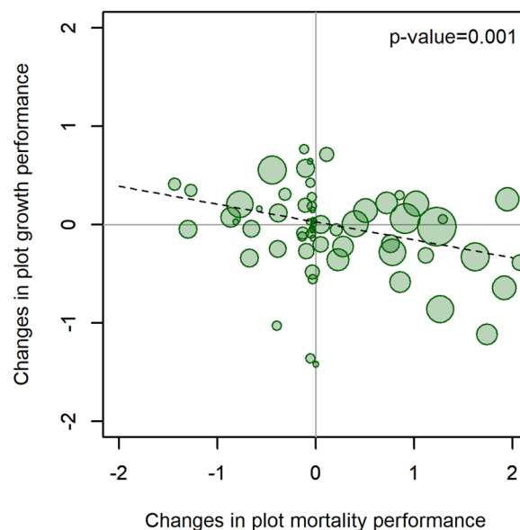
Figure 5. Plot level changes along time in ash tree mortality compared to growth performance. The changes are presented using the differences between the estimated plot random factors for mortality and growth in the period 2010–14 compared to the initial period 2000–04. The size of the circles represents the number of ash trees per plot.
