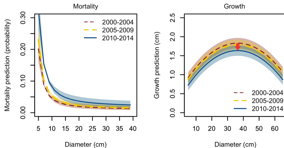
Figure 2. Modelled probability of ash tree mortality and growth. Mortality (left) and growth (right) predictions presented according to the tree diameter and for the three periods studied (2000–04, 2005–09, 2010–14, corresponding to the 8 th , 9 th and 10 th national forest inventories, respectively). The earliest detection of ash dieback in Norway corresponds to the period (2005–09) and the disease is supposed to have spread along the west coast of the country in the latest period (2010–14). The models show the predictions for the median basal area (BA) on the mortality predictions and median basal area of larger trees (BAL) for the growth predictions. The shadowed areas represent the thresholds for the first and third quartile (BA = 19–31 m 2 ha -1 and BAL = 12–25.2 m 2 ha -1 respectively). The arrow illustrates the average growth reduction along inventories.
