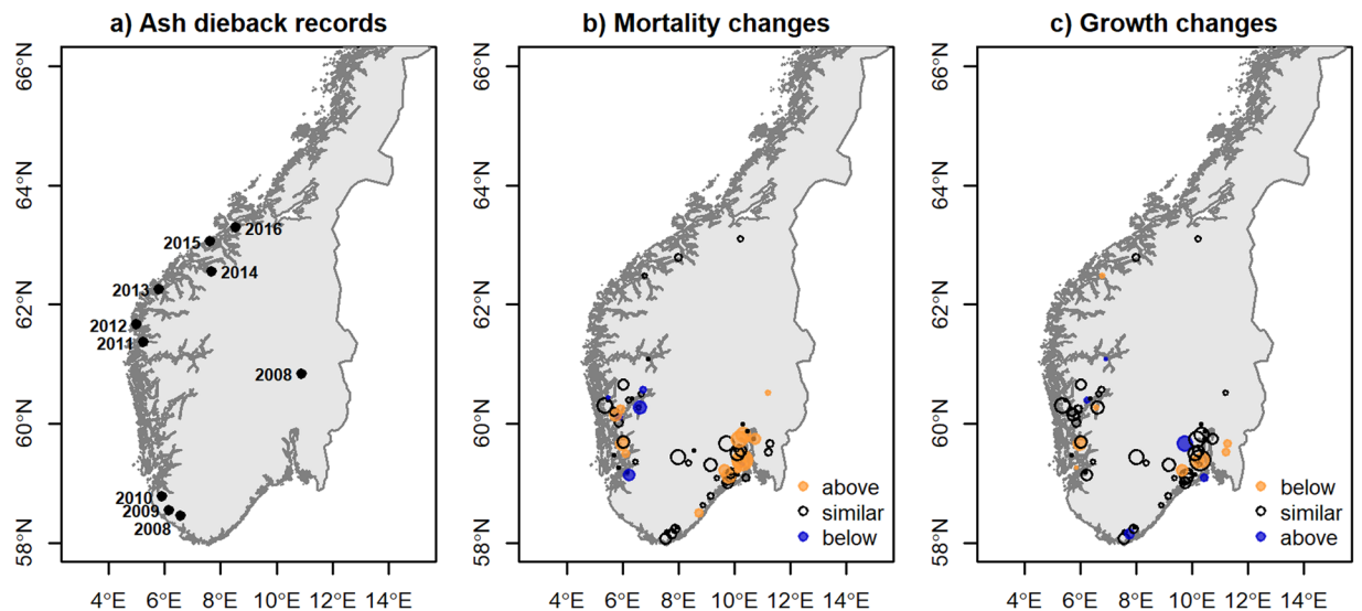
Figure 4. Changes in estimated plot mortality and growth. (A) Illustrates the first year of identification of the disease as a reference, the data is from ash dieback records from targeted inventories 24 . (B) Shows the mortality changes in a plot from the estimates of the random factors for the period 2010–14 compared to the period 2000–04 (Eq. 1) and (C) Shows the growth changes in a plot (Eq. 2). The values considered to be similar are within one standard deviation. The size of the circles represents the number of ash trees per plot. Maps generated with R ( www.R-project.org ); layer retrieved from ©Kartverket N250 ( www.kartverket.no ).
