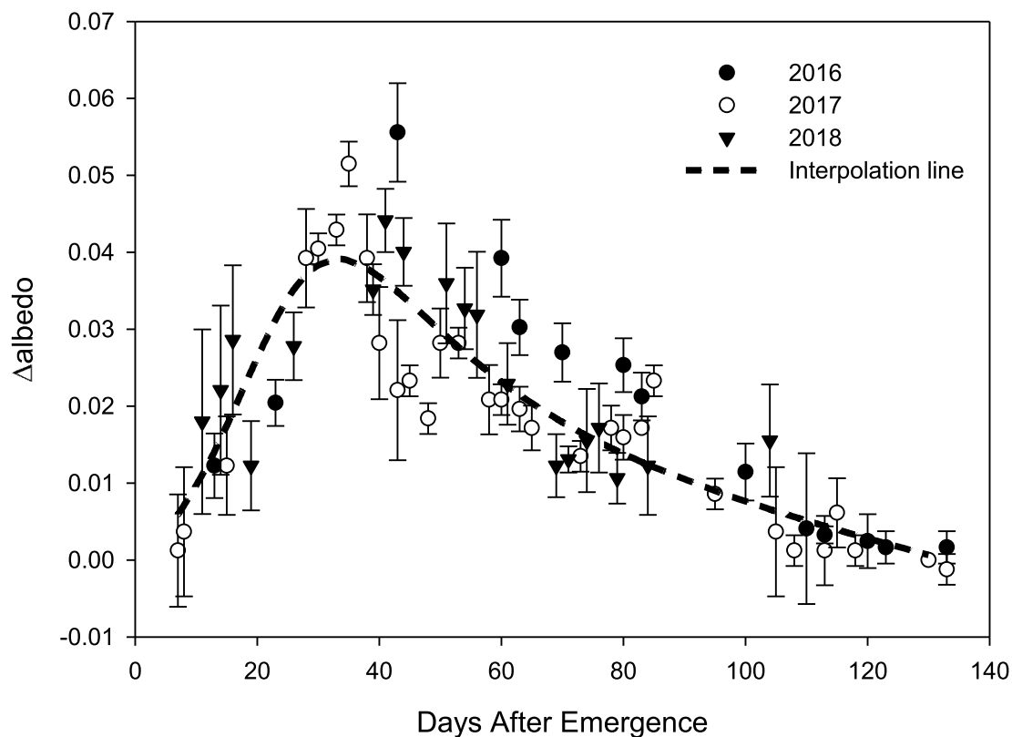
Figure 4. Differences in surface daily albedo ( \Delta albedo) between MinnGold and the commercial soybean varieties estimated from Sentinel 2 satellite data in Udine in 2016 ( n = 14 ), 2017 ( n = 31 ) and 2018 ( n = 19 ). The interpolation line was obtained by means of a modified skewed Pearson probability density function. The variability of satellite values within plots is presented as standard deviation (vertical bars).
