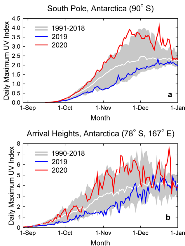
Fig. 1 Daily maximum UV index (UVI) measured at the South Pole (a) and Arrival Heights (b) in 2019 (blue line) and 2020 (red line), compared with the average (white line) and the range (grey shading) of daily maximum observations of the years indicated in the legends. The UVI was calculated from spectra measured by SUV-100 spectroradiometers. Up to 2009, the instruments were part of the NSF UV monitoring network [13] and they are now a node in the NOAA Antarctic UV Monitoring Network ( https://www.esrl.noaa.gov/gmd/grad/antuv/ ). Consistent data processing methods were applied for all years [14, 15]. In 2020, the UVI was typically above the long-term average at both sites due to the sustained and deep stratospheric ozone hole in that year. Conversely, the UVI in 2019 was close to the lower limit of historical observations because warming of the Antarctic stratosphere produced one of the smallest ozone holes on record in that year [1, 8]
